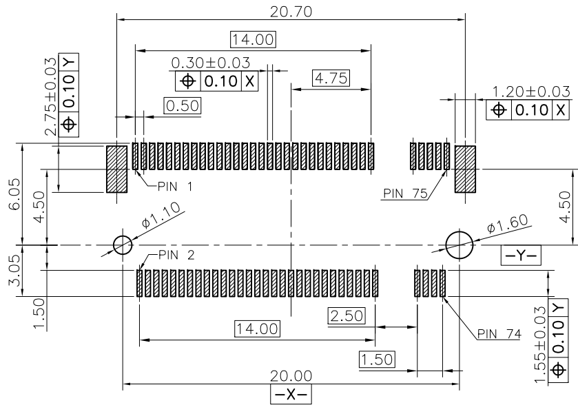
Recommended PCB Layout (Top View) Default Tolerance ±0.05
