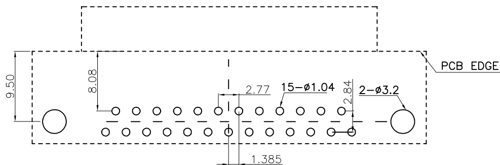
PCB LAYOUT
