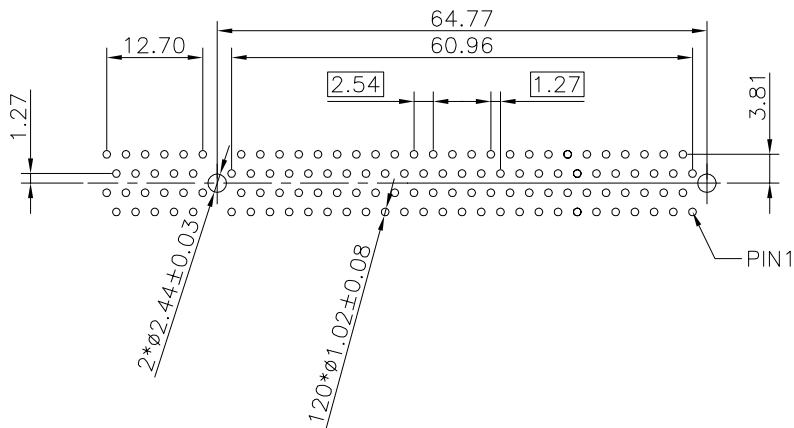
RECOMMENDED PCB LAYOUT DEFAULT TOLERANCE ±0.05
