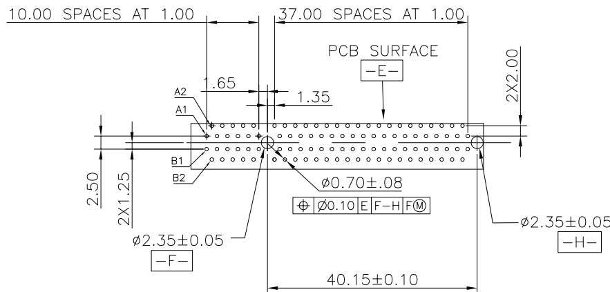
RECOMMENDED PCB LAYOUT DEFAULT TOLERANCE ±0.05
